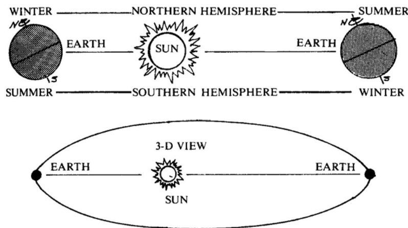
Figure 9 - Orbital Heating Changes
