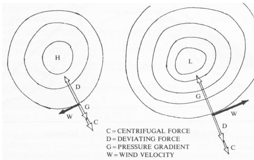
Forces Around Pressure Systems
