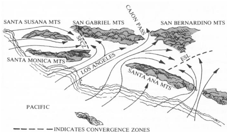
Figure 159 - Convergence on Complex Terrain Near the Sea
